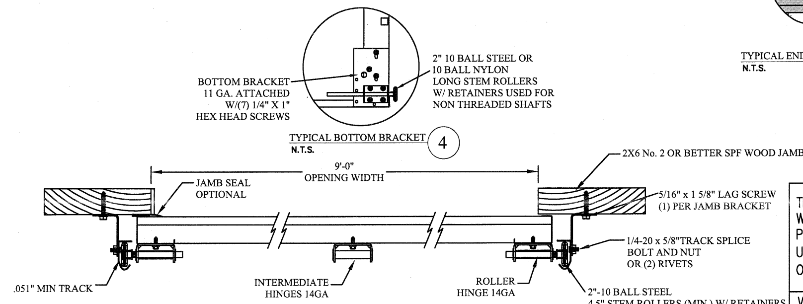
2" BRACKET MOUNT TO WOOD JAMB DETAIL
